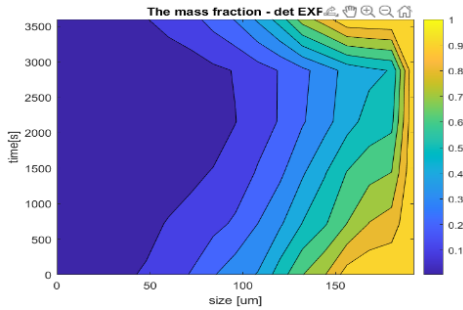
Figure 6 The contour lines of the experimentally determined cumulative mass fraction
